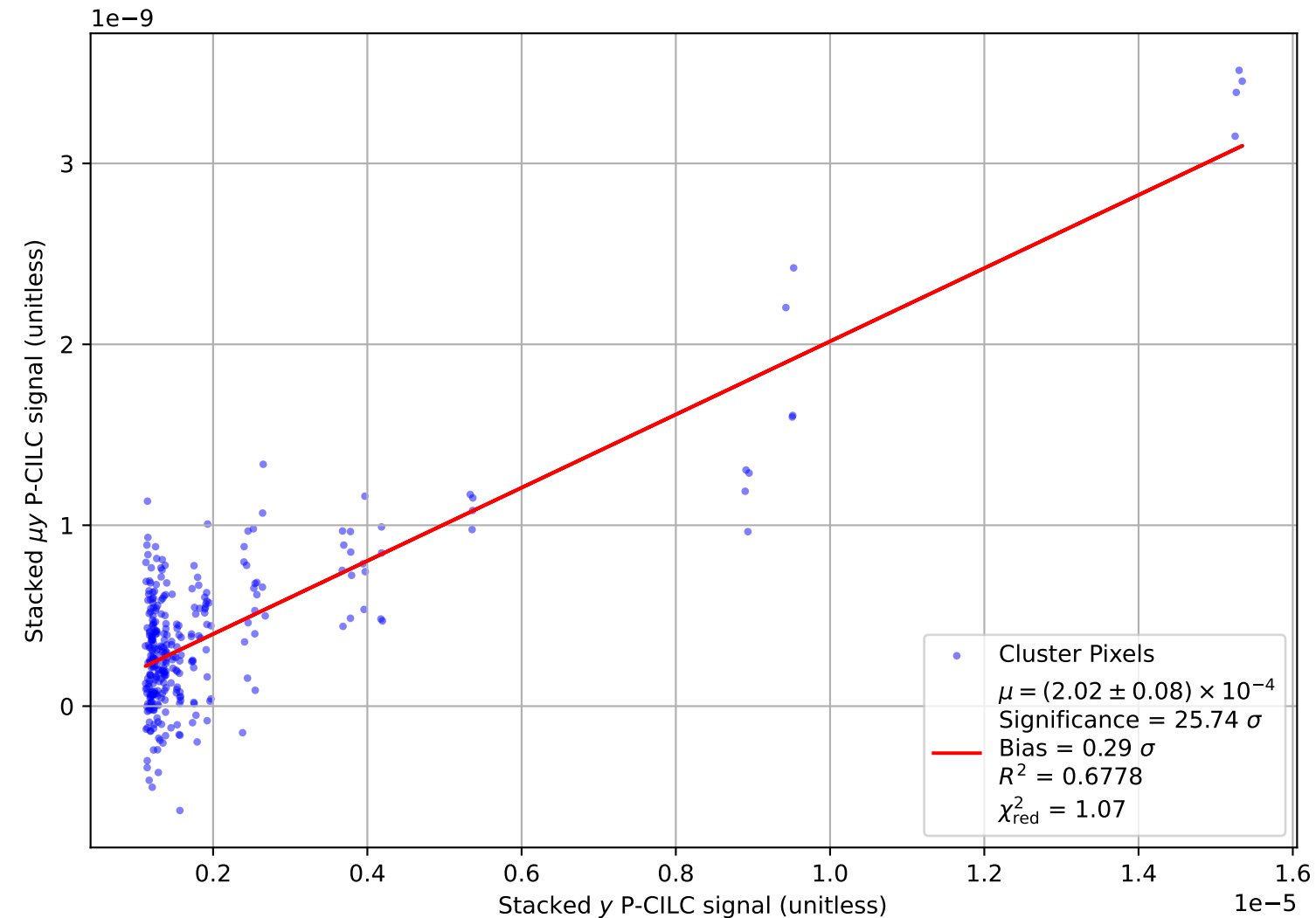
T-T Plot: P-CILC \mu y Vs. P-CILC y , \mu = 2\text{e-}04 , base sensitivity = 0.20 \mu\text{K}\cdot\text{arcmin} , r \leq 10 pixels, PICO
