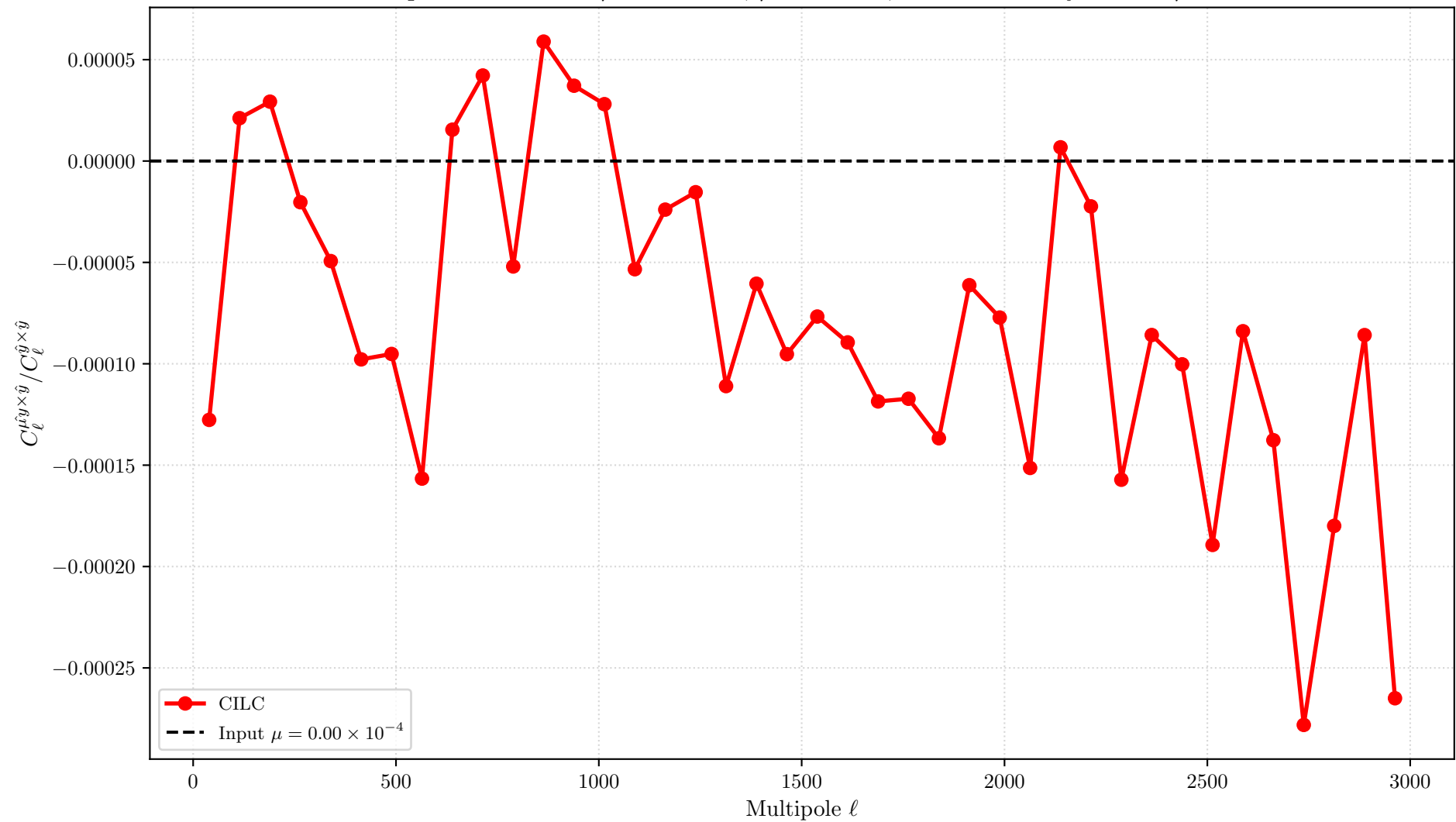
Binned spectral ratio for \mu extraction, \mu = 0\text{e}+00 , base sensitivity = 0.61 \mu\text{K}\cdot\text{arcmin}
