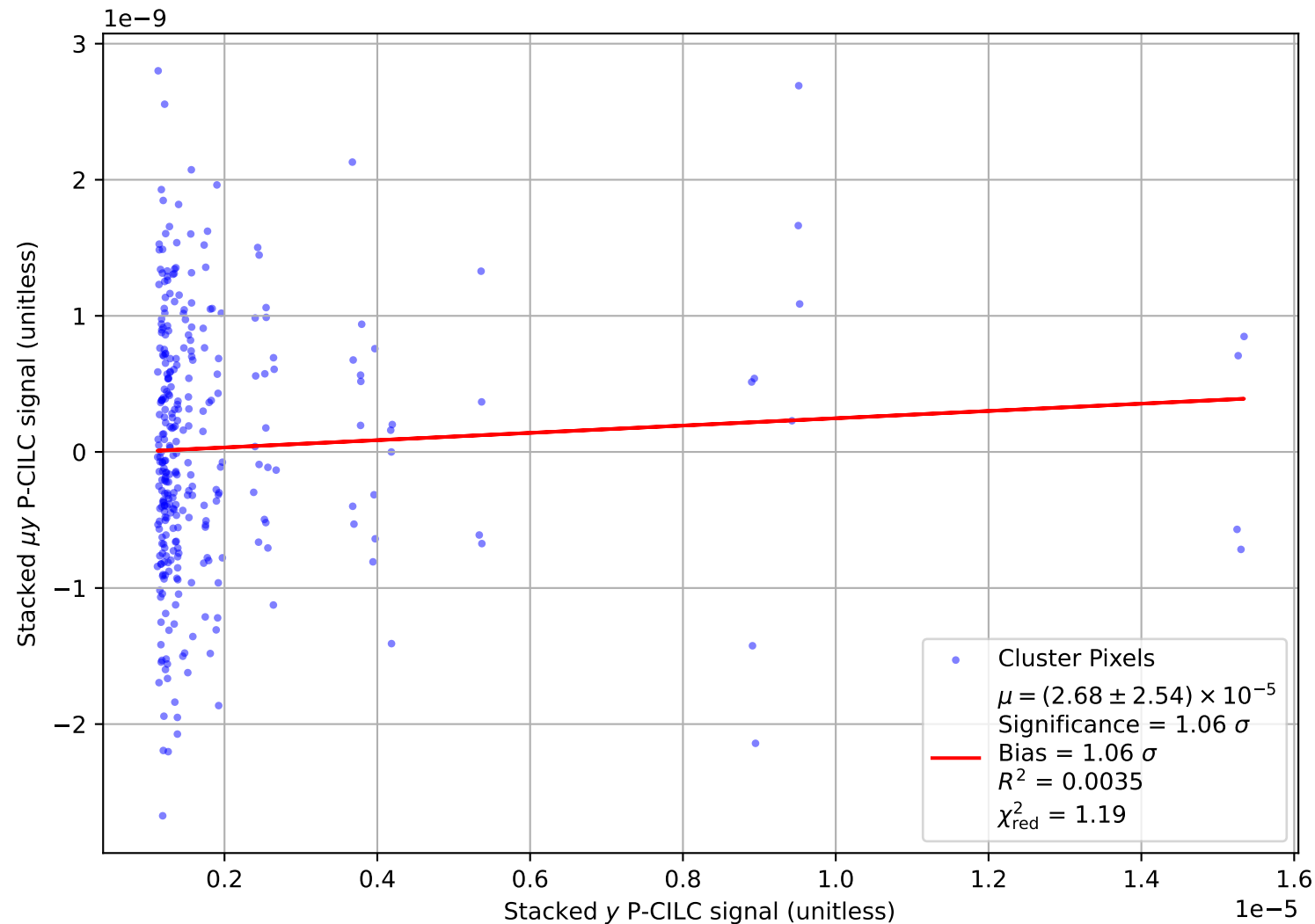
T-T Plot: P-CILC \mu y Vs. P-CILC y , \mu = 0\text{e}+00 , base sensitivity = 0.61 \mu\text{K}\cdot\text{arcmin} , r \leq 10 pixels
