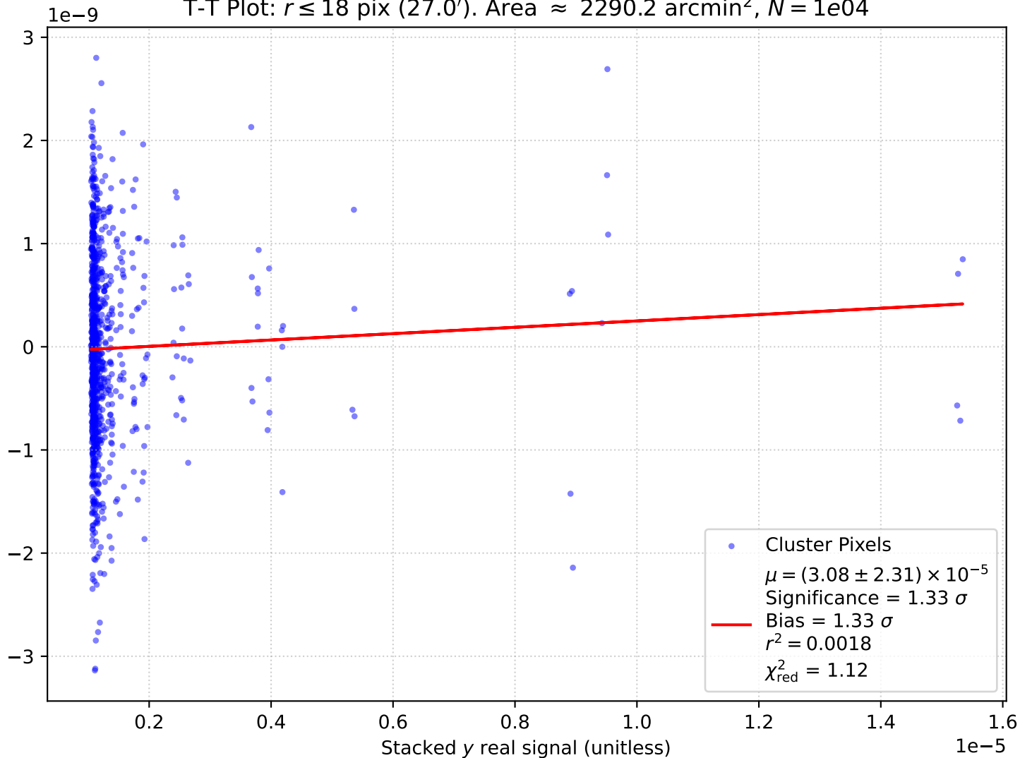
T-T Plot: r \leq 18 pix (27.0'). Area \approx 2290.2 arcmin 2 , N = 1e04
