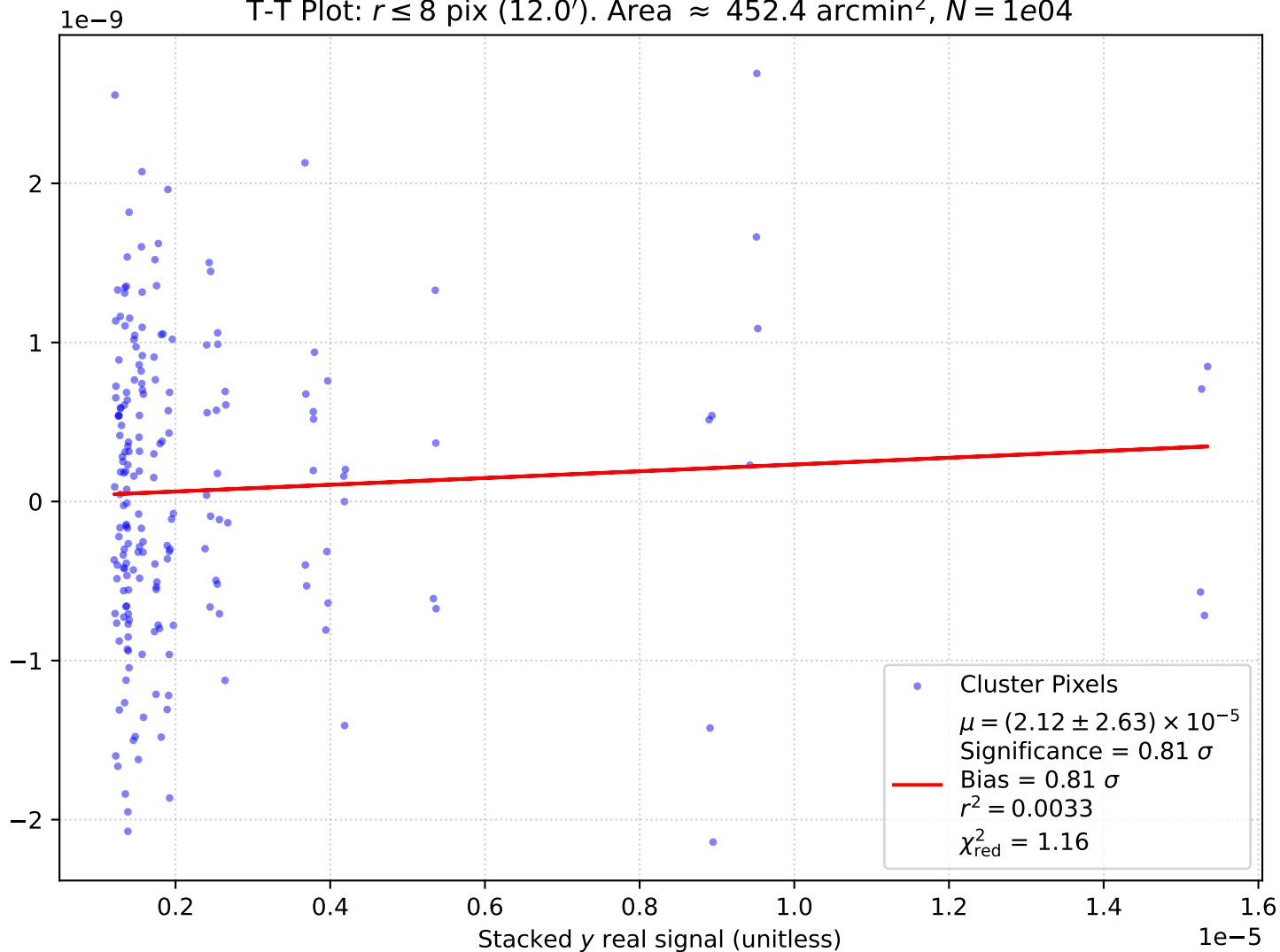
T-T Plot: r \leq 8 pix (12.0'). Area \approx 452.4 arcmin 2 , N = 1e04
