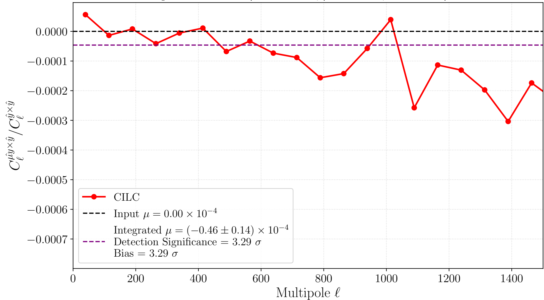
Binned spectral ratio for \mu extraction, \mu = 0\text{e}+00 , s_n = 0.20 \mu\text{K}\cdot\text{arcmin}
