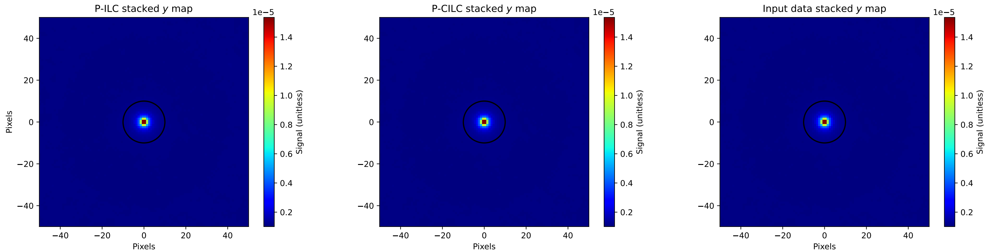
Comparison of y map stacked patches of 1\text{e}+04 brightest clusters, \mu value = 2\text{e}-04 , base sensitivity = 0.20\ \mu\text{K}\cdot\text{arcmin} , r = 10\text{p}
