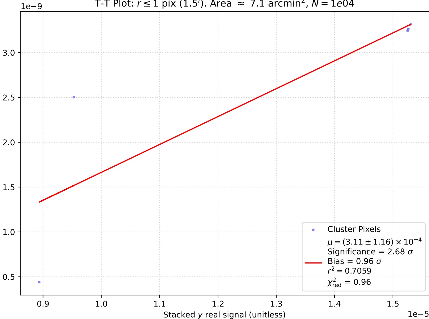
T-T Plot: r \leq 1 pix (1.5'). Area \approx 7.1 arcmin 2 , N = 1e04
