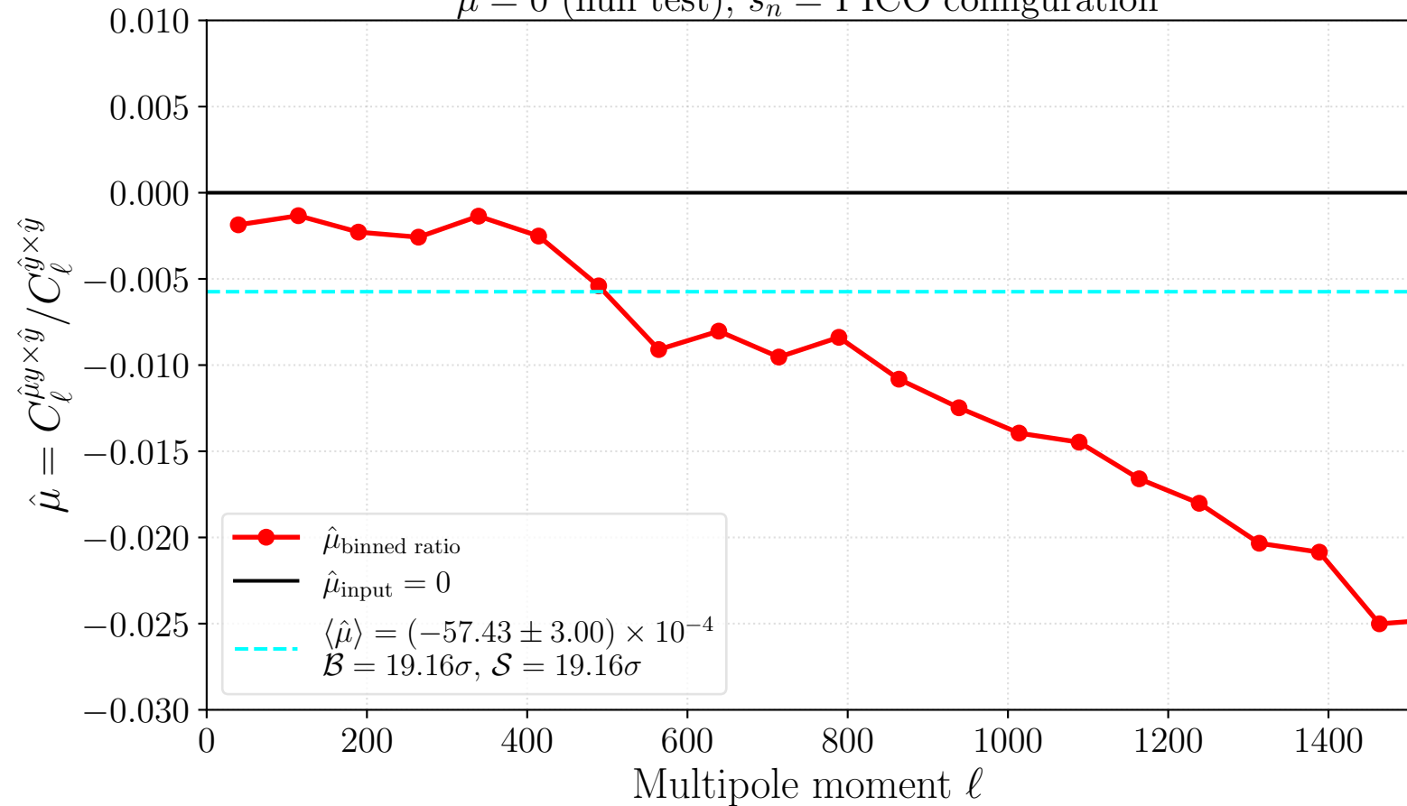
Binned spectral ratio for \mu extraction, PICO configuration, \mu = 0 (null test), s_n = \text{PICO configuration}
