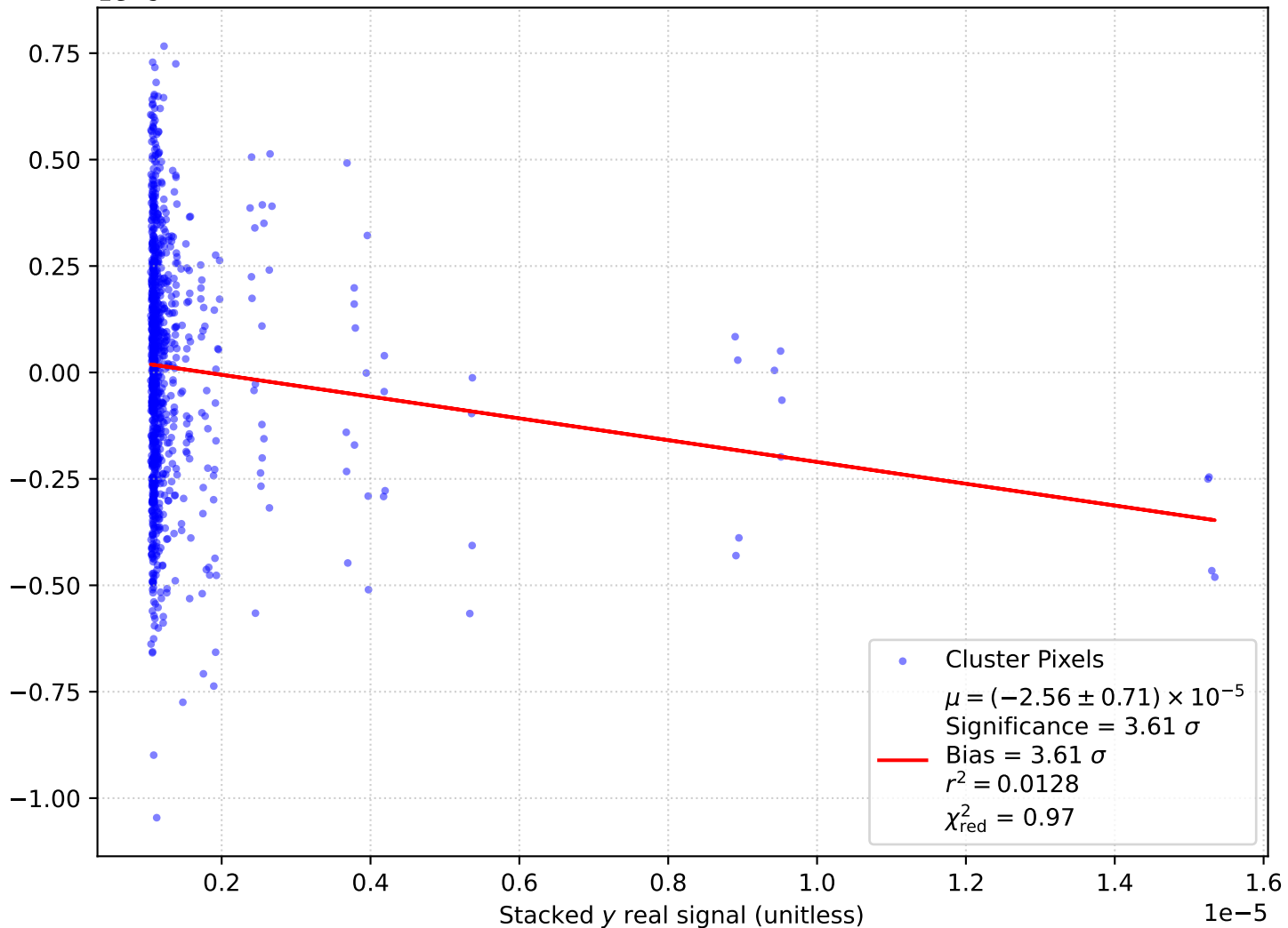
T-T Plot: r \leq 18 pix (27.0'). Area \approx 2290.2 arcmin 2 , N = 1e04
