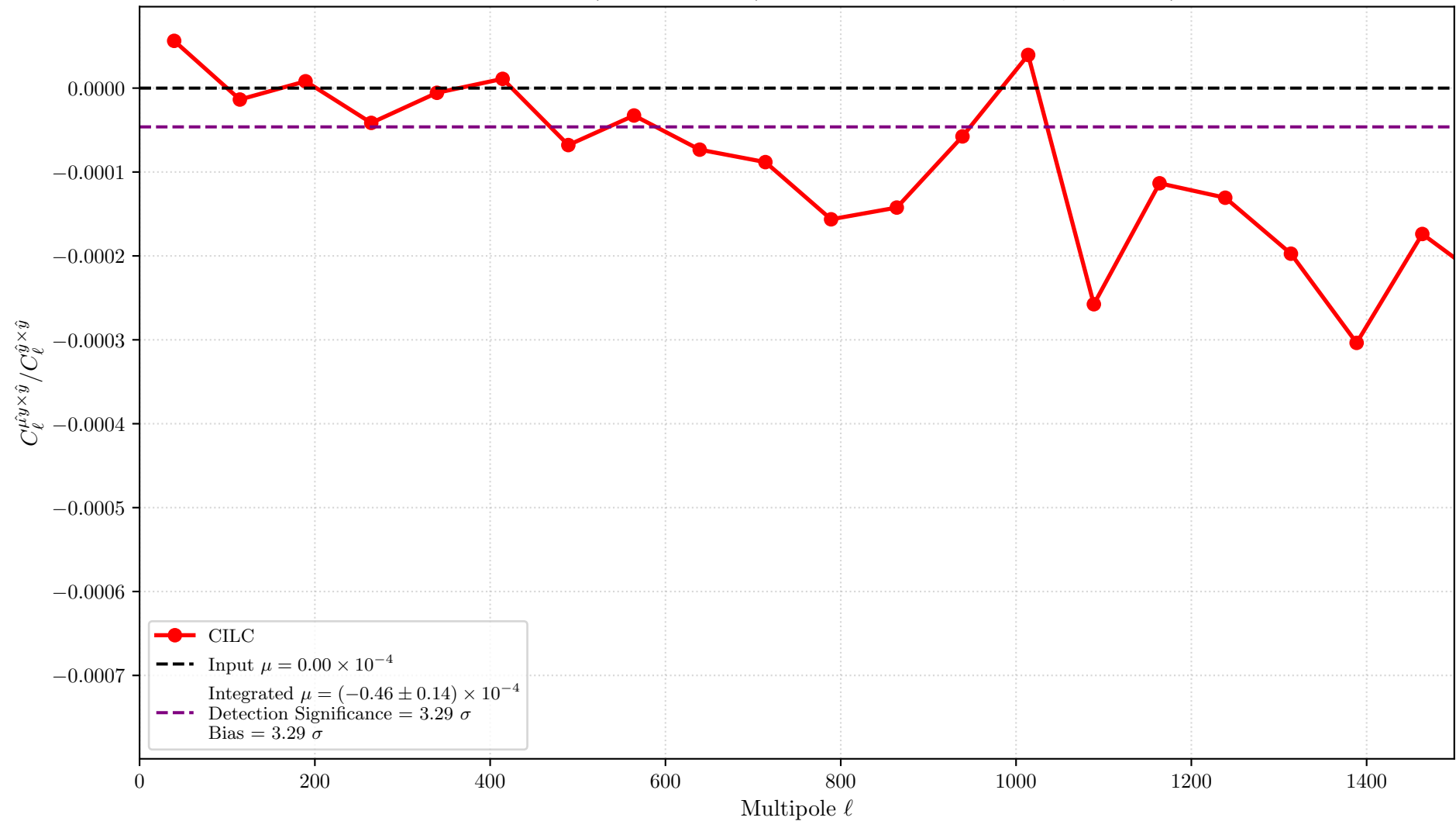
Binned spectral ratio for \mu extraction, \mu = 0\text{e}+00 , base sensitivity = 0.20 \mu\text{K}\cdot\text{arcmin}
