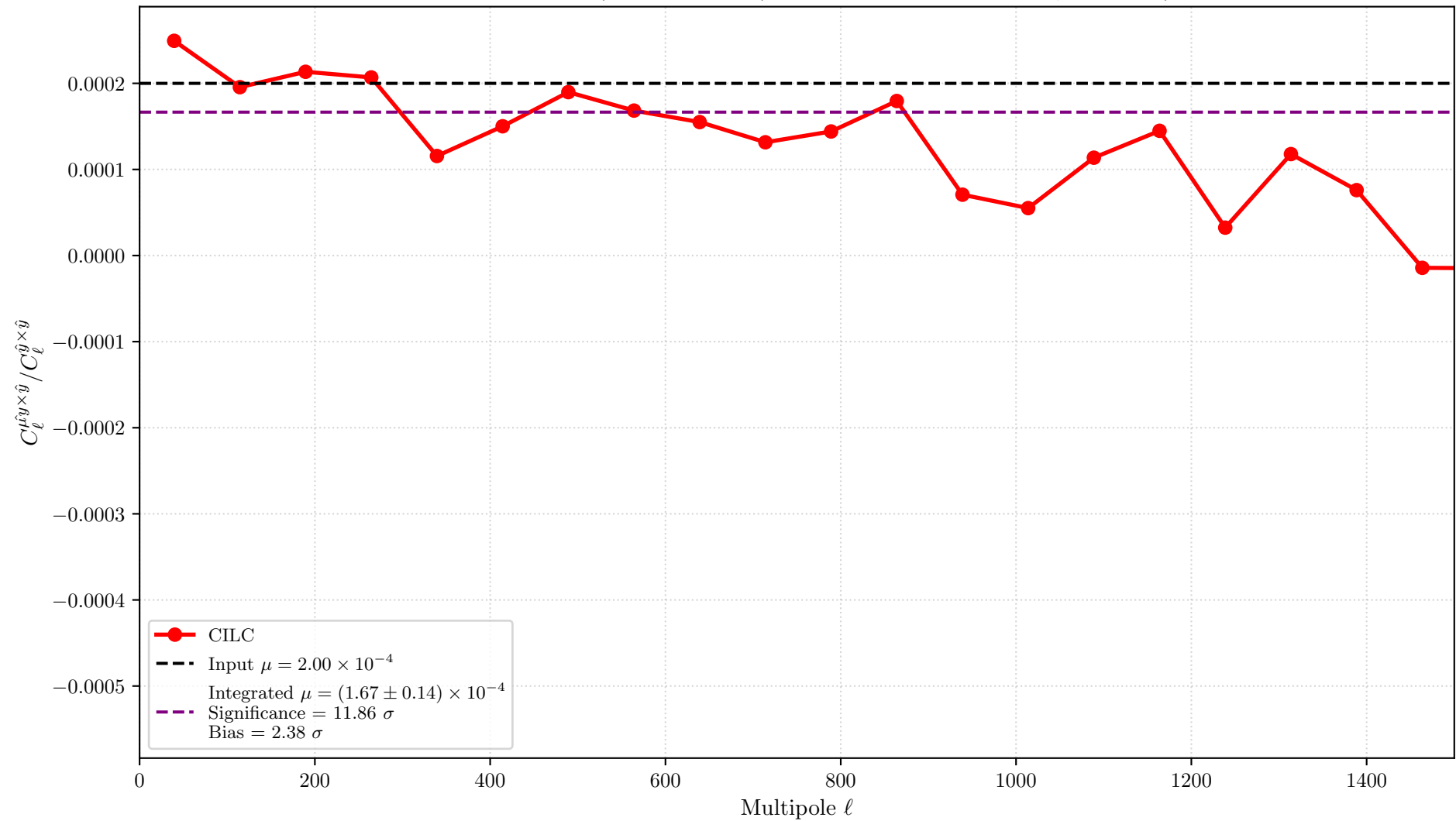
Binned spectral ratio for \mu extraction, \mu = 2\text{e-}04 , base sensitivity = 0.20 \mu\text{K}\cdot\text{arcmin}
