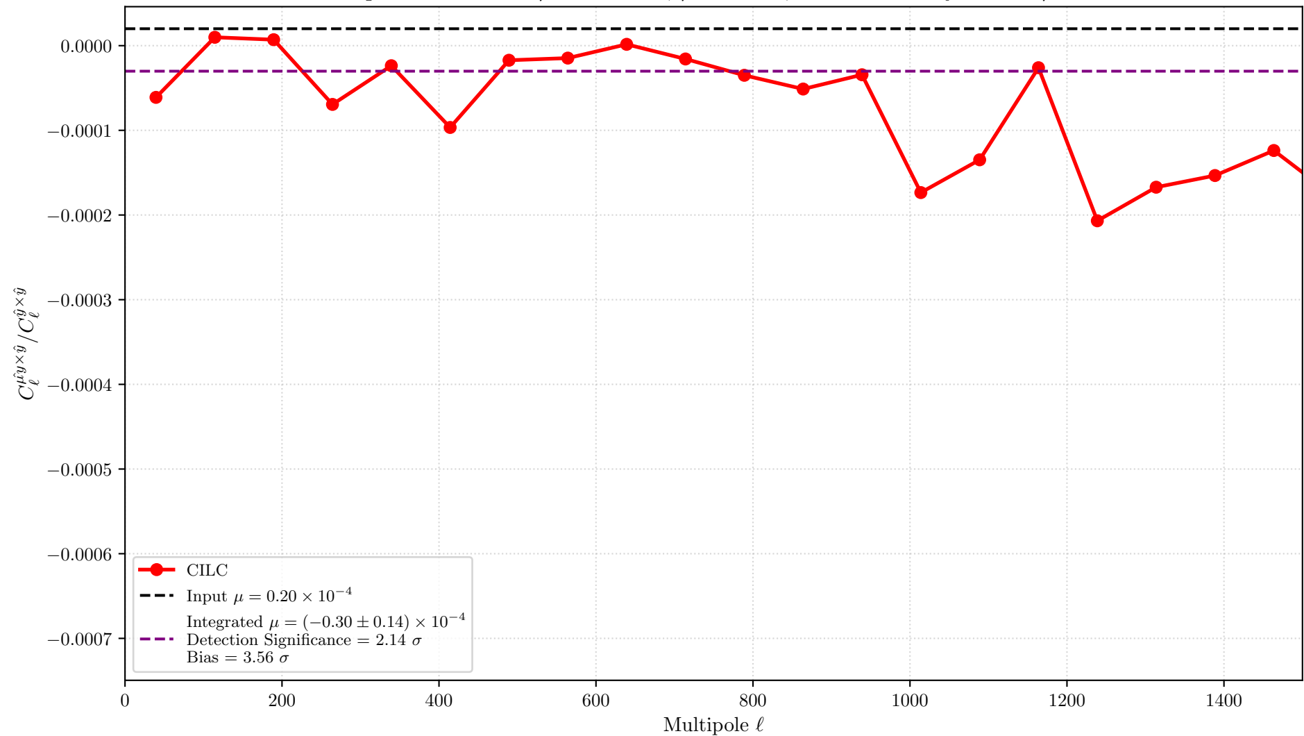
Binned spectral ratio for \mu extraction, \mu = 2\text{e-}05 , base sensitivity = 0.20 \mu\text{K}\cdot\text{arcmin}
