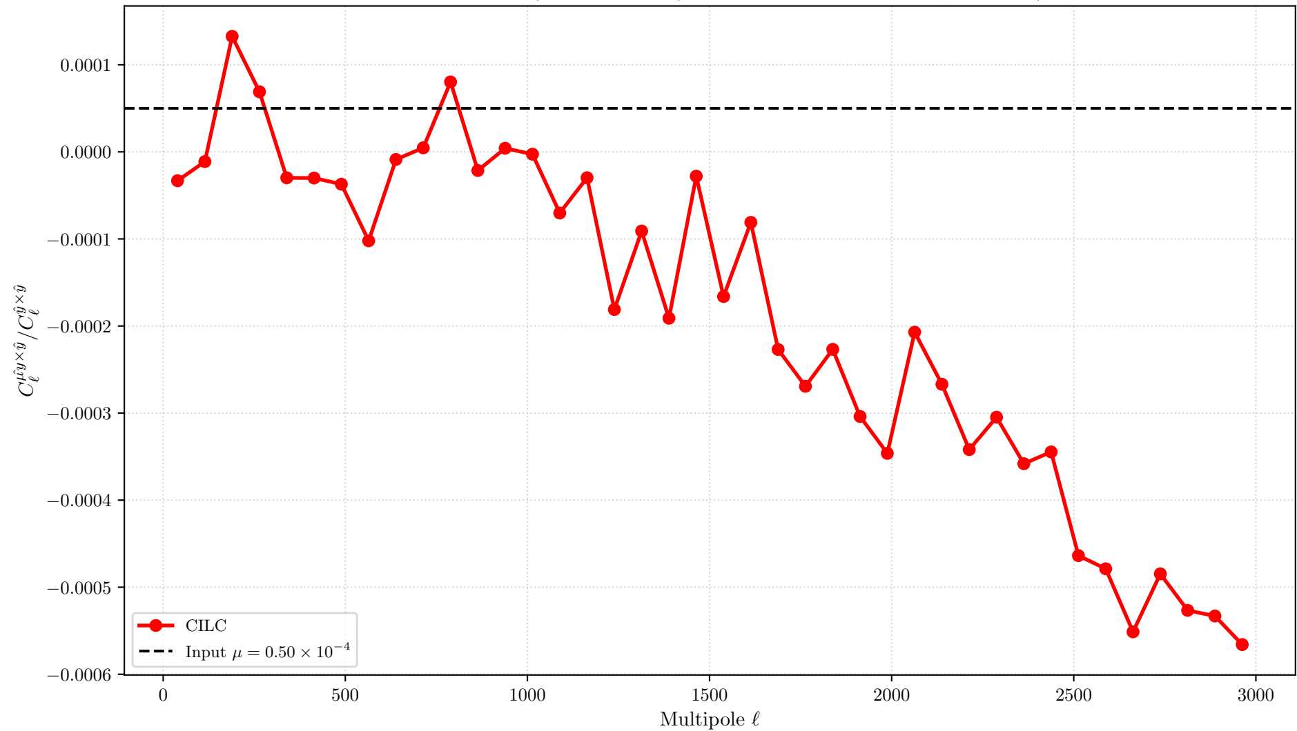
Binned spectral ratio for \mu extraction, \mu = 5\text{e-}05 , base sensitivity = 0.20 \mu\text{K}\cdot\text{arcmin}
