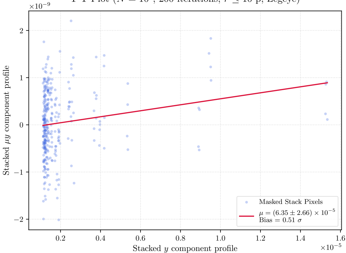
T-T Plot ( N = 10^4 , 200 iterations, r \leq 10 p, Zegeye)
