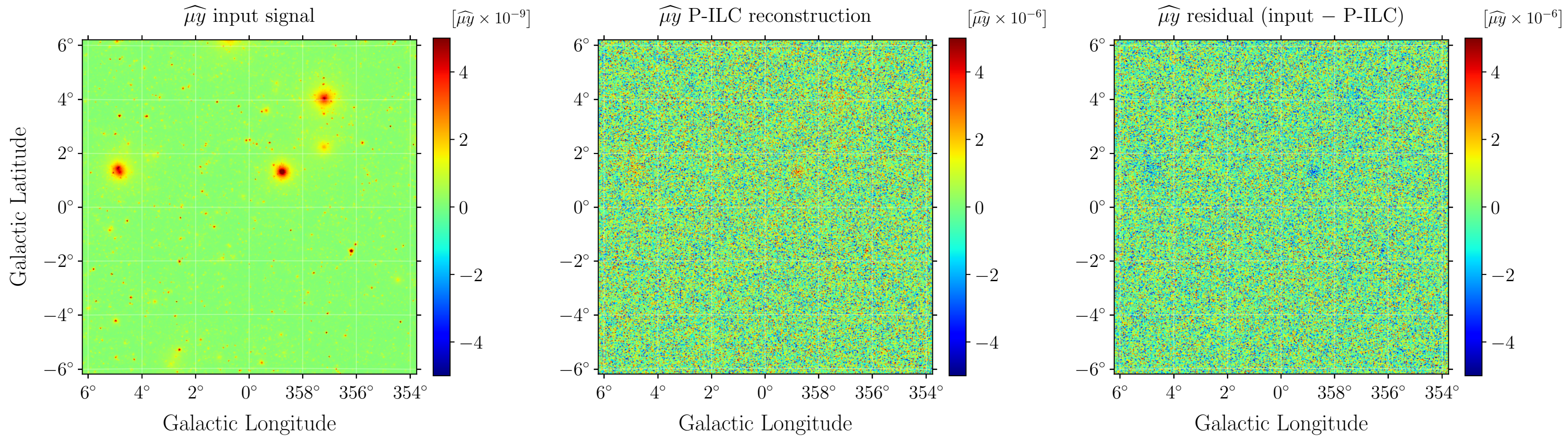
Zoomed Input Map and P-ILC reconstructed and residual \widehat{\mu y} maps, \mu = 2 \times 10^{-4} , PICO configuration
