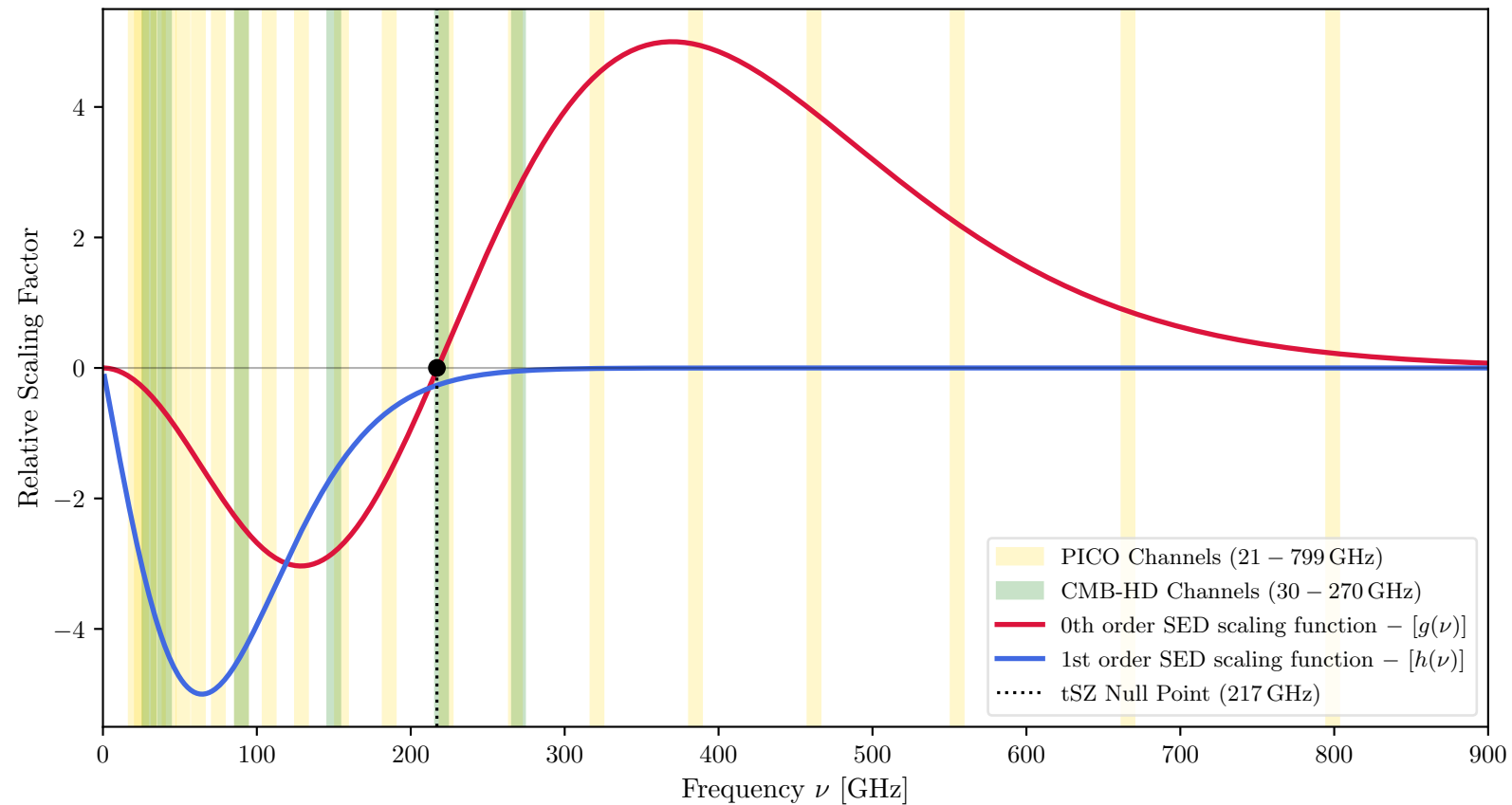
g(\nu) and h(\nu) frequency scaling in intensity units (normalized)
