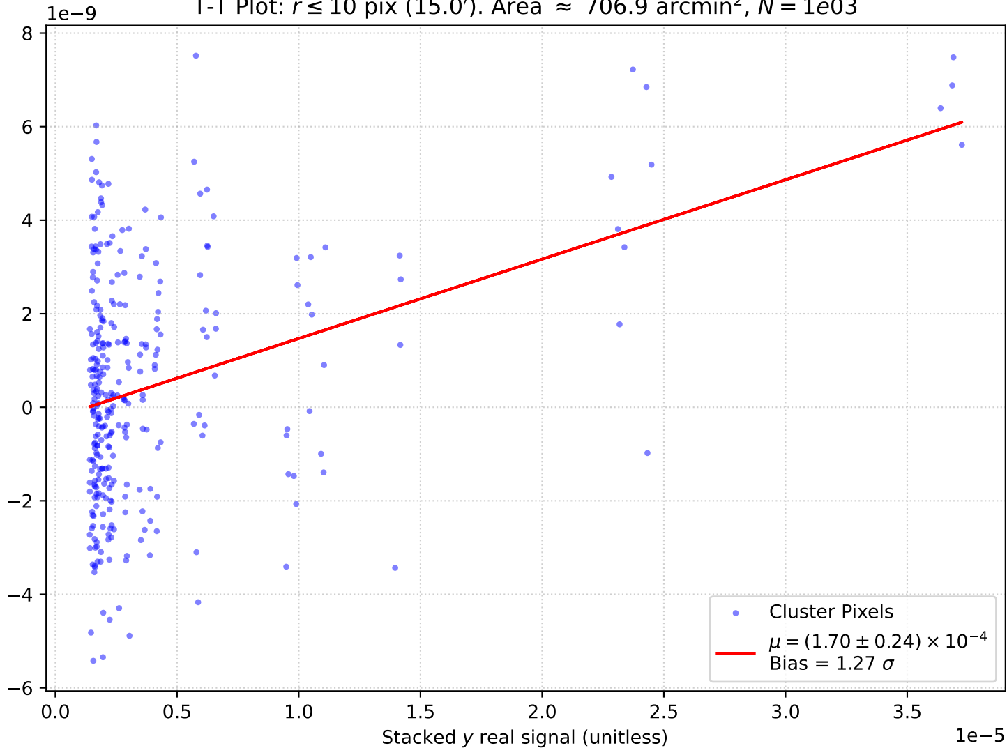
T-T Plot: r \leq 10 pix (15.0'). Area \approx 706.9 arcmin 2 , N = 1e03
