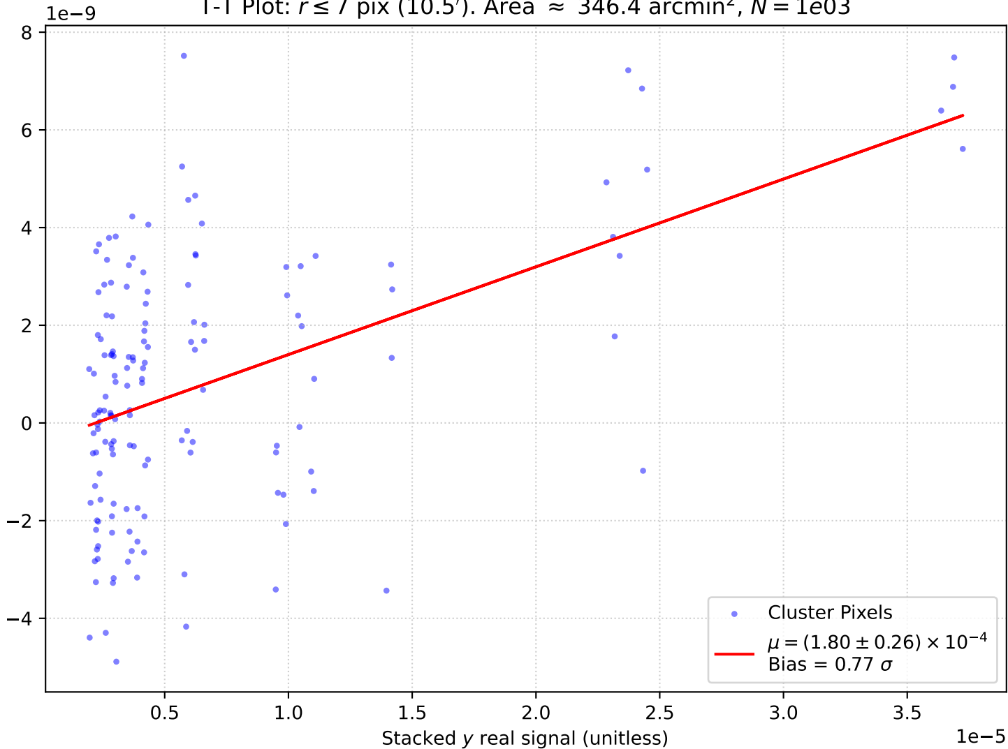
T-T Plot: r \leq 7 pix (10.5'). Area \approx 346.4 arcmin 2 , N = 1e03
