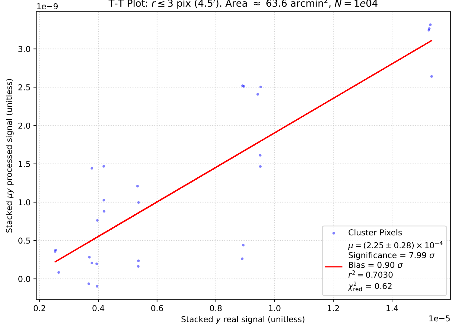
T-T Plot: r \leq 3 pix (4.5'). Area \approx 63.6 arcmin 2 , N = 1e04
