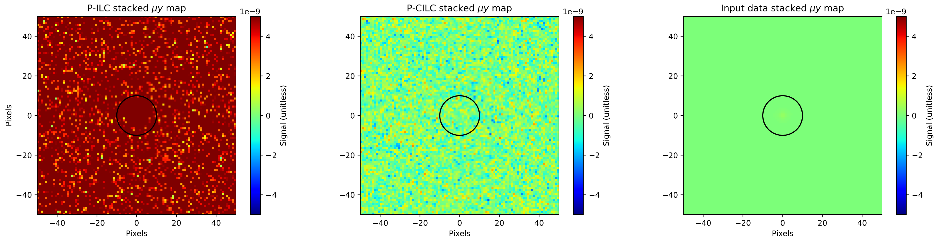
Comparison of \mu y map stacked patches of 1e+04 brightest clusters, \mu value = 2e-05 , base sensitivity = 0.20 \mu K \cdot \text{arcmin} , r = 10p
