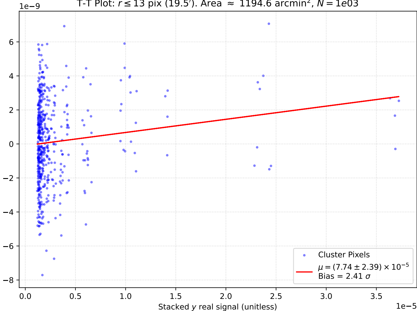
T-T Plot: r \leq 13 pix (19.5'). Area \approx 1194.6 arcmin 2 , N = 1e03
