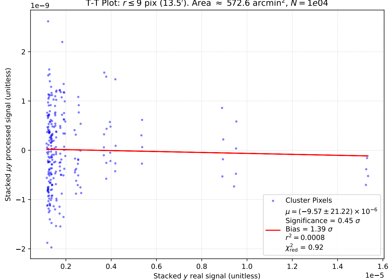
T-T Plot: r \leq 9 pix (13.5'). Area \approx 572.6 arcmin 2 , N = 1e04
