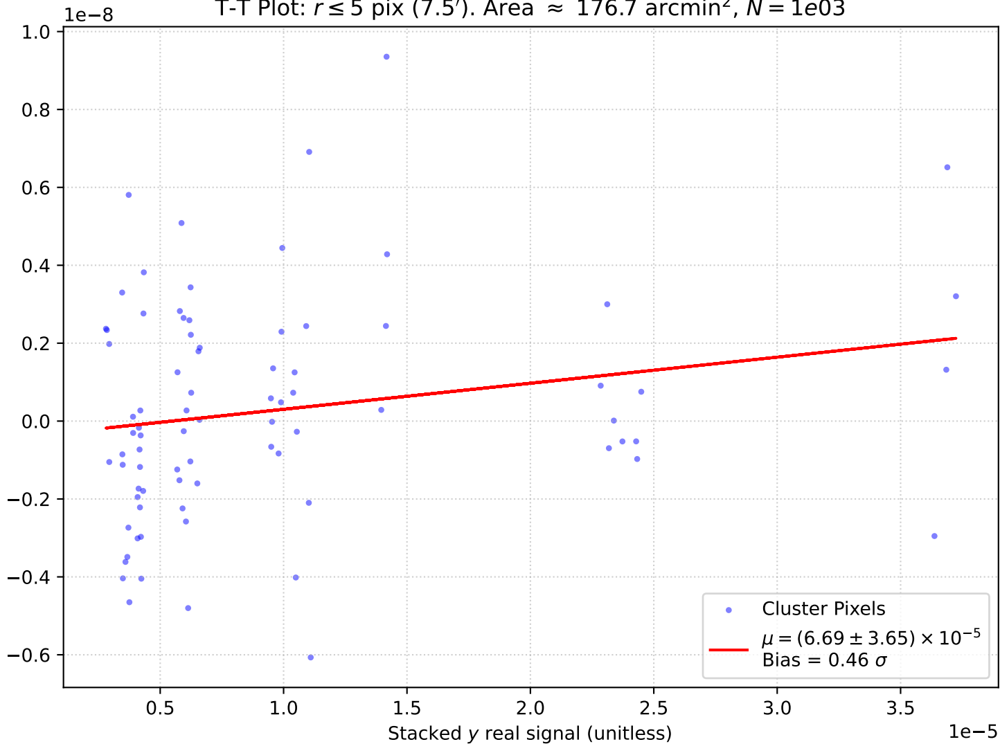
T-T Plot: r \leq 5 pix (7.5'). Area \approx 176.7 arcmin 2 , N = 1e03
