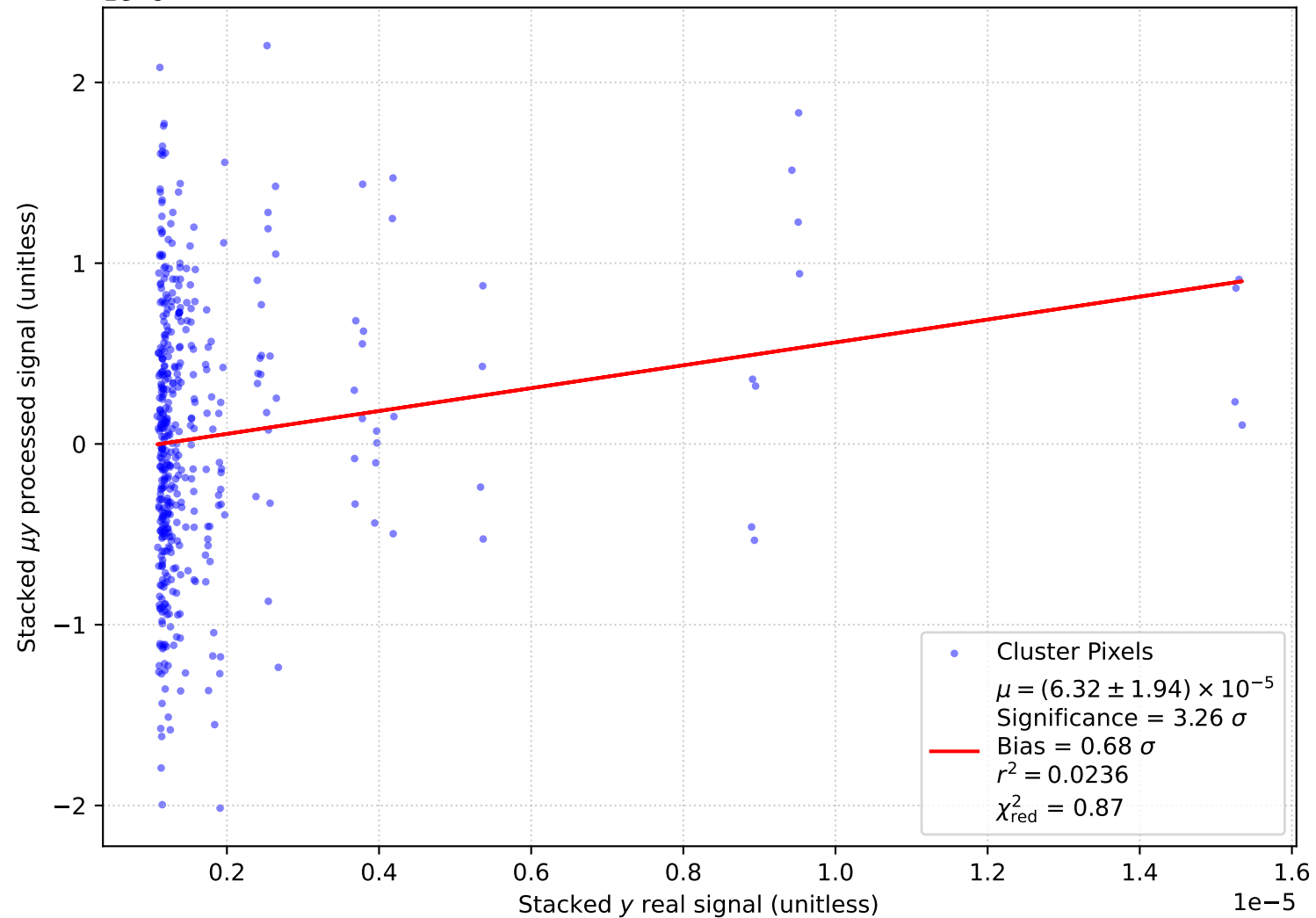
T-T Plot: r \leq 12 pix (18.0'). Area \approx 1017.9 arcmin 2 , N = 1e04
