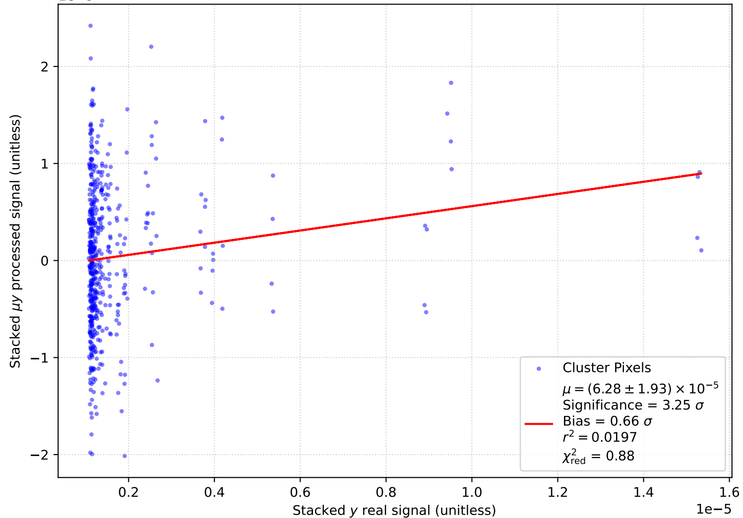
T-T Plot: r \leq 13 pix (19.5'). Area \approx 1194.6 arcmin 2 , N = 1e04
