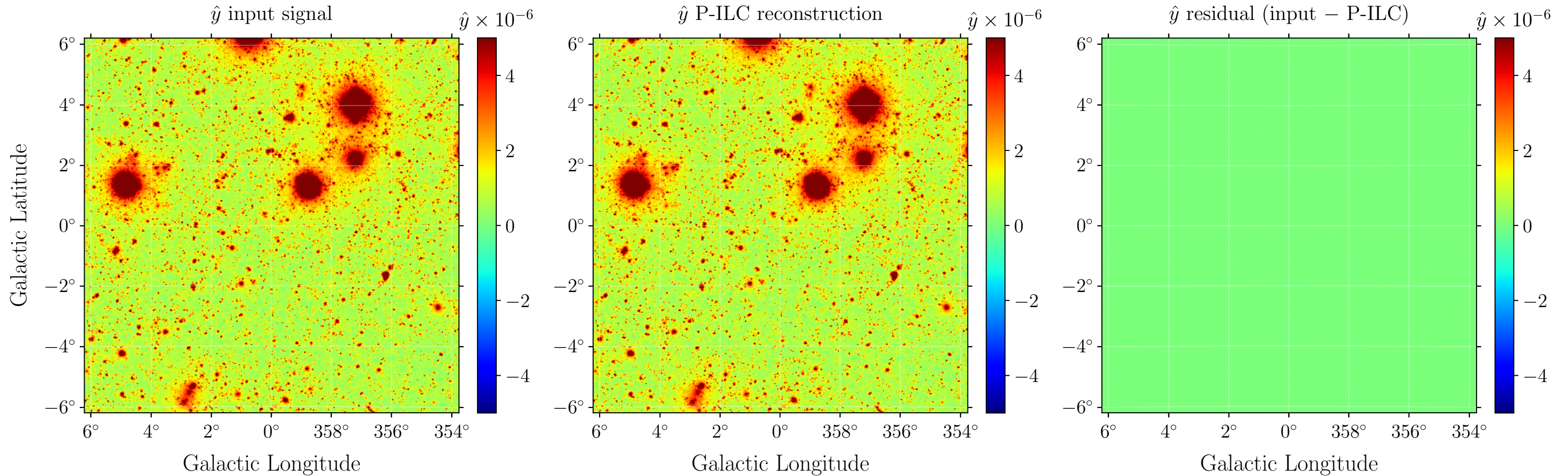
Zoomed input map and P-ILC reconstructed and residual \hat{y} maps, \mu = 2 \times 10^{-4} , PICO-like configuration, s_n = 0.2 \mu\text{K} \cdot \text{arcmin}
