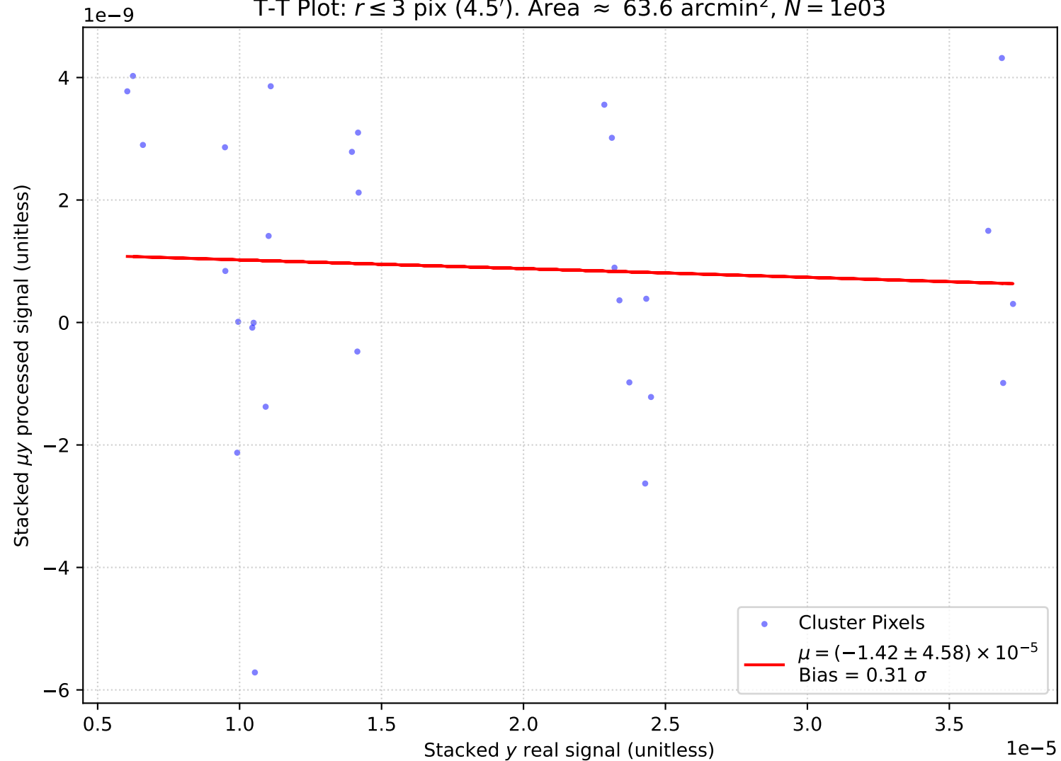
T-T Plot: r \leq 3 pix (4.5'). Area \approx 63.6 arcmin 2 , N = 1e03
