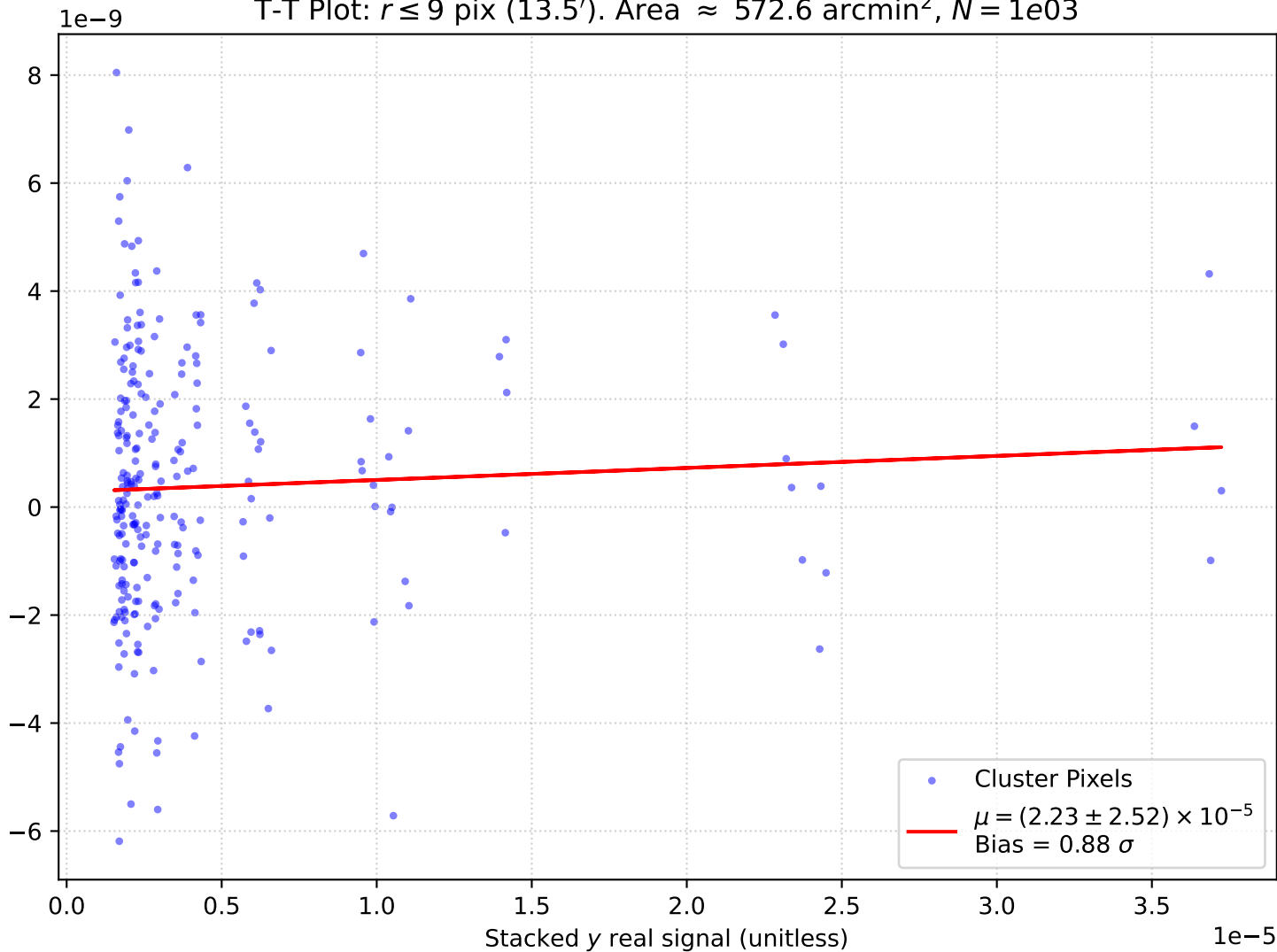
T-T Plot: r \leq 9 pix (13.5'). Area \approx 572.6 arcmin 2 , N = 1e03
