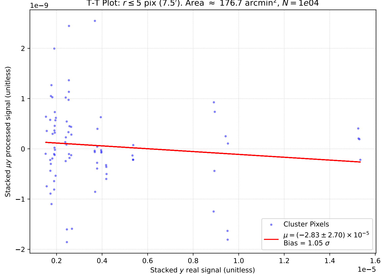
T-T Plot: r \leq 5 pix (7.5'). Area \approx 176.7 arcmin 2 , N = 1e04
