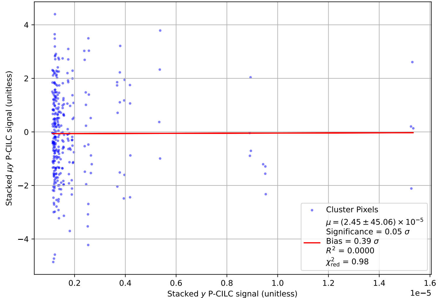
T-T Plot: P-CILC \mu y Vs. P-CILC y , \mu = 2\text{e-}04 , base sensitivity = PICO, r \leq 10 pixels, PICO 1e-8
