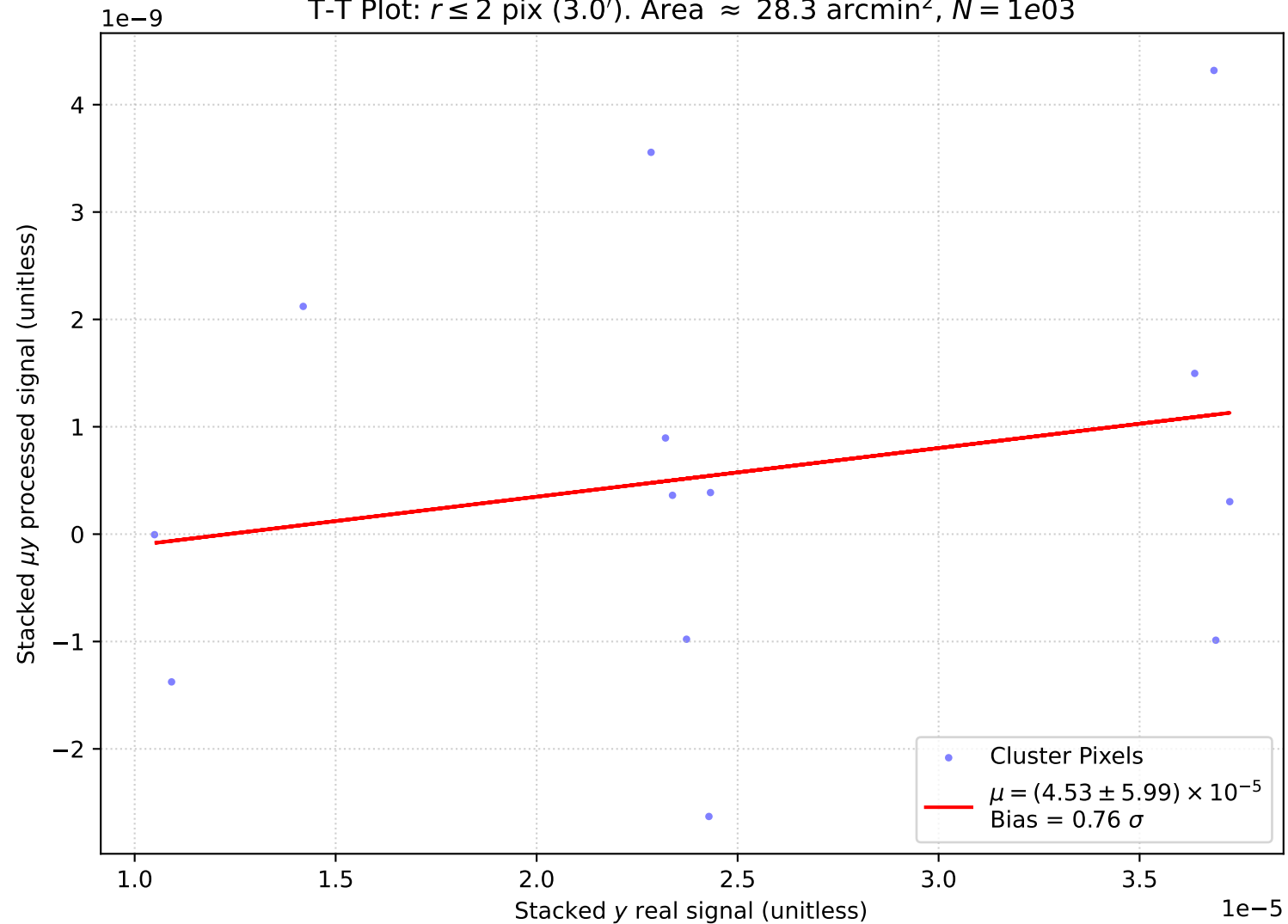
T-T Plot: r \leq 2 pix (3.0'). Area \approx 28.3 arcmin 2 , N = 1e03
