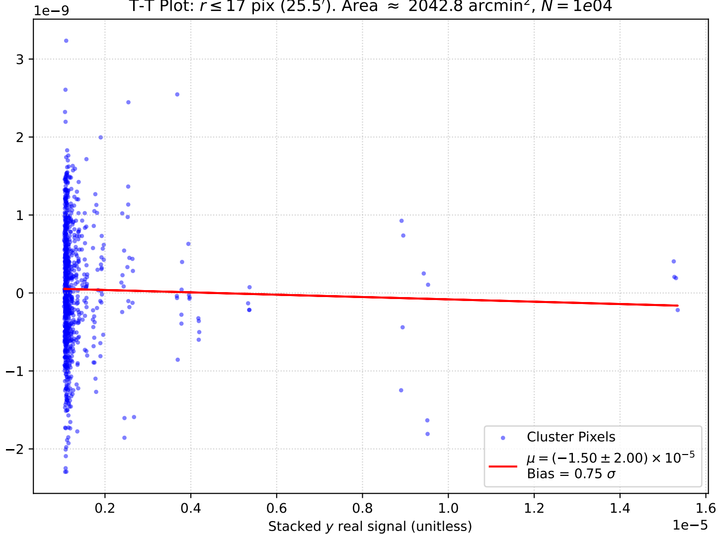
T-T Plot: r \leq 17 pix (25.5'). Area \approx 2042.8 arcmin 2 , N = 1e04
