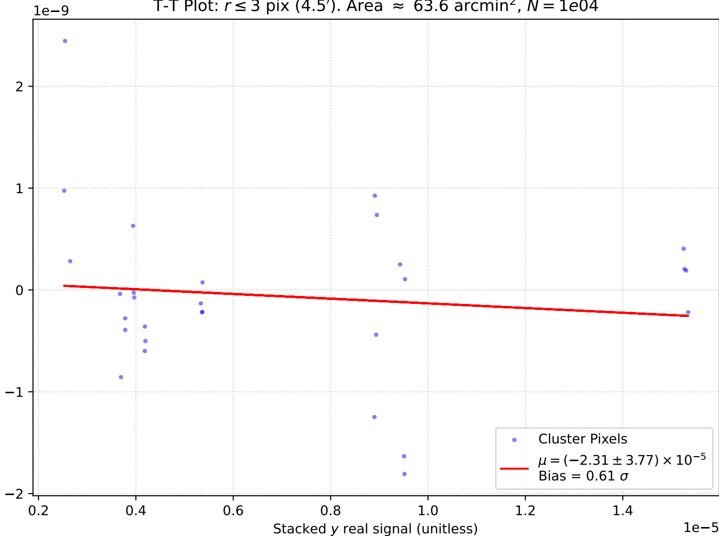
T-T Plot: r \leq 3 pix (4.5'). Area \approx 63.6 arcmin 2 , N = 1e04
