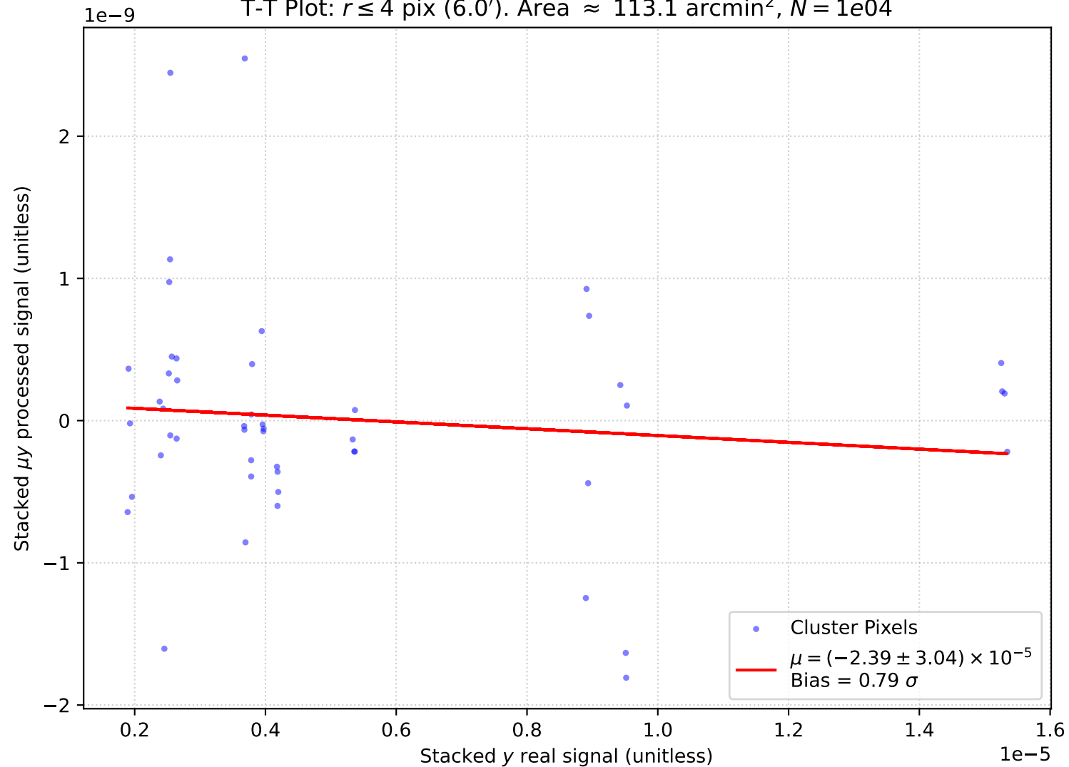
T-T Plot: r \leq 4 pix (6.0'). Area \approx 113.1 arcmin 2 , N = 1e04
