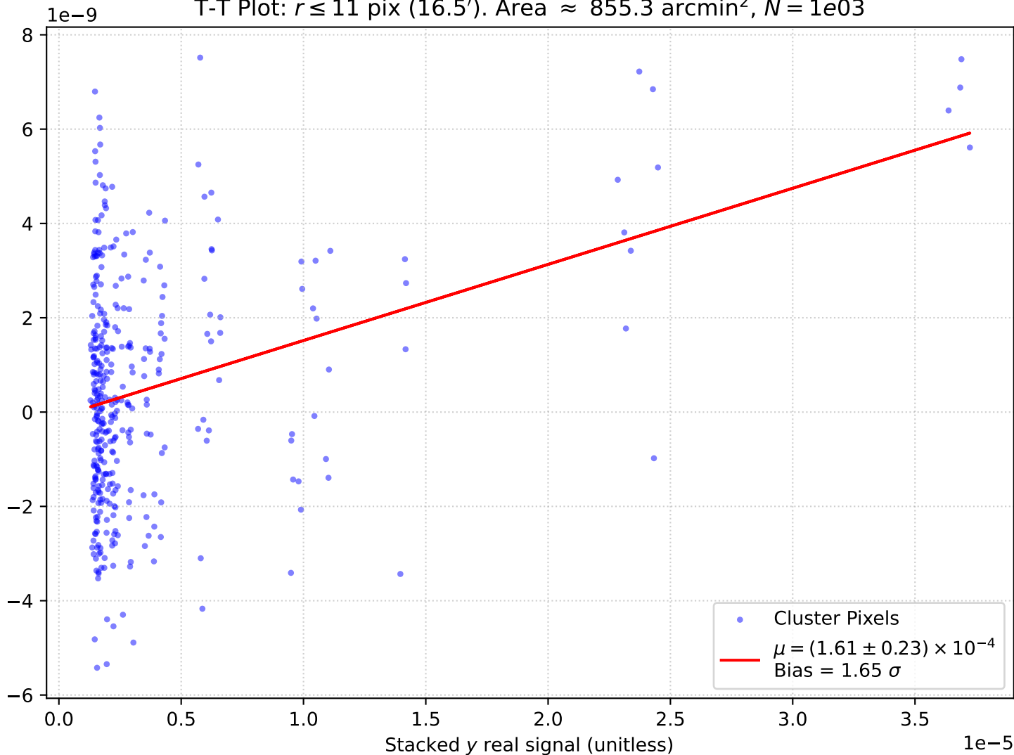
T-T Plot: r \leq 11 pix (16.5'). Area \approx 855.3 arcmin 2 , N = 1e03
