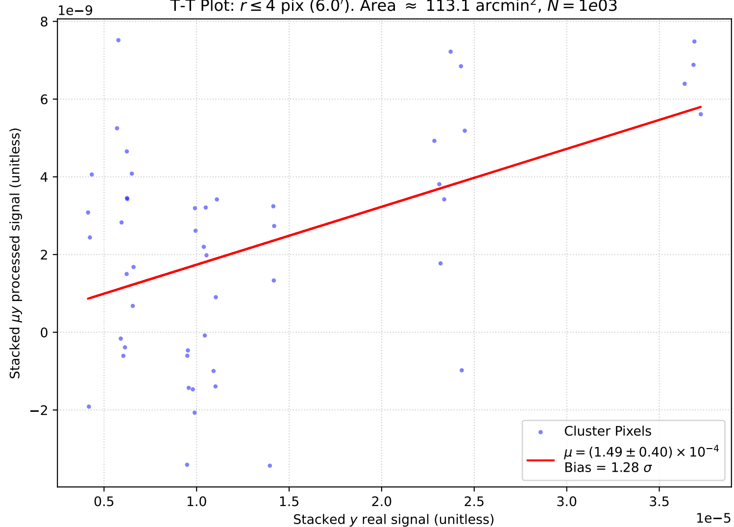
T-T Plot: r \leq 4 pix (6.0'). Area \approx 113.1 arcmin 2 , N = 1e03
