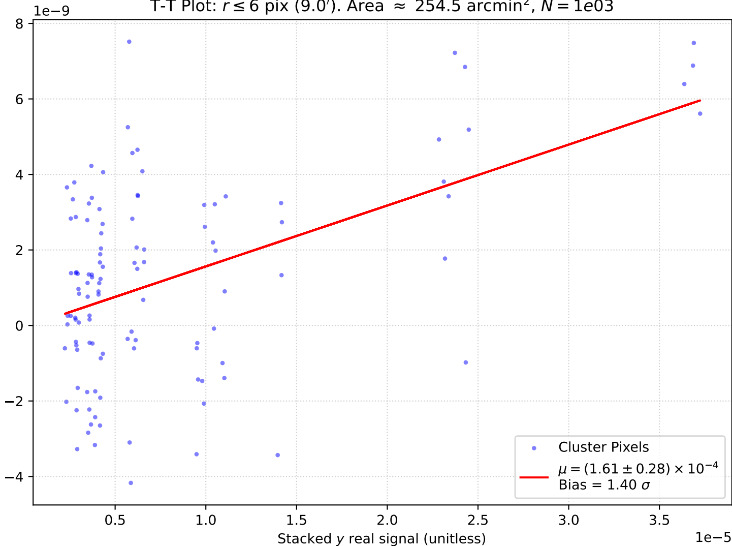
T-T Plot: r \leq 6 pix (9.0'). Area \approx 254.5 arcmin 2 , N = 1e03
