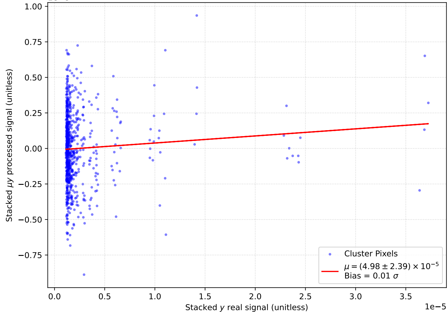
T-T Plot: r \leq 16 pix (24.0'). Area \approx 1809.6 arcmin 2 , N = 1e03
