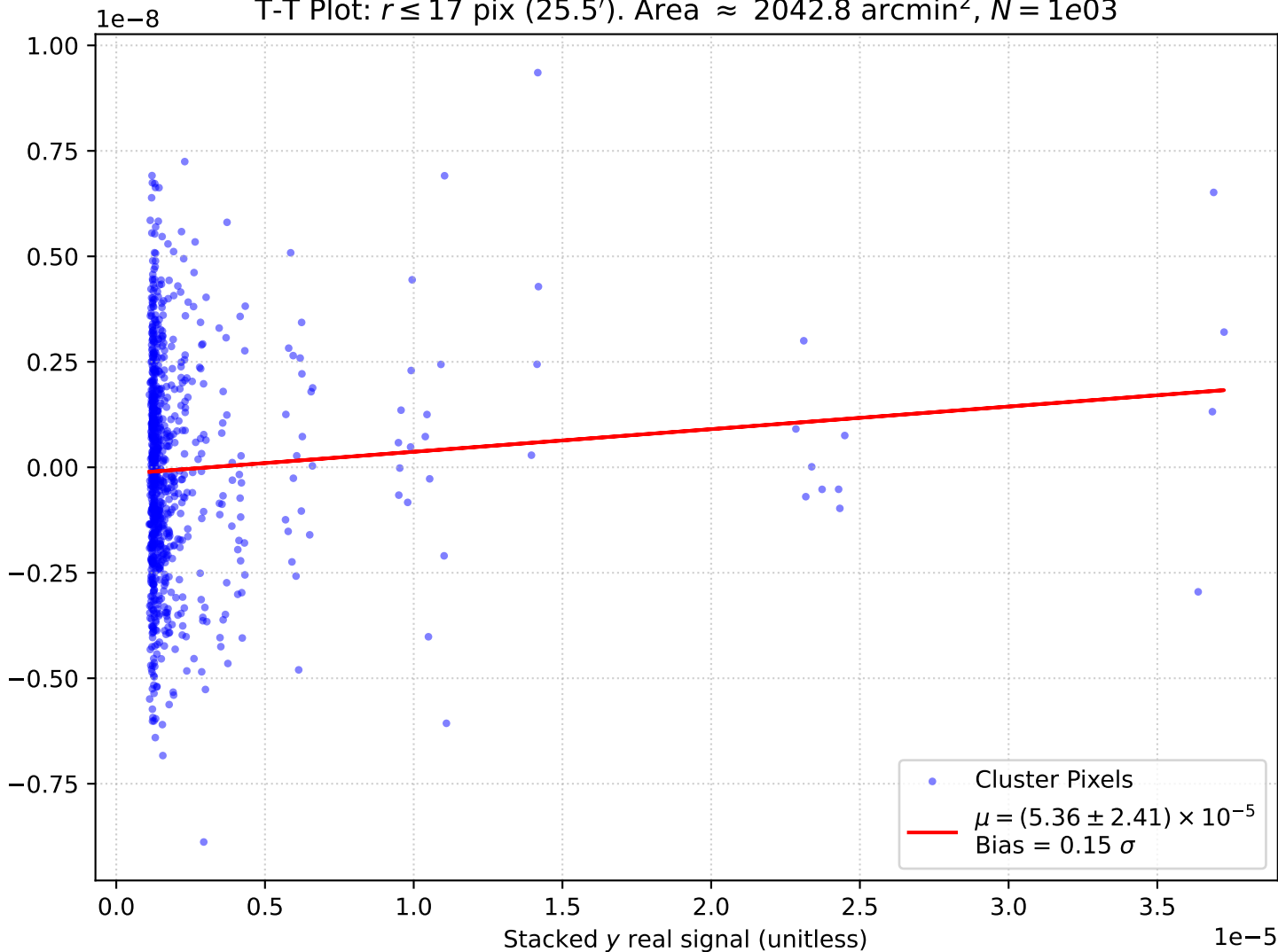
T-T Plot: r \leq 17 pix (25.5'). Area \approx 2042.8 arcmin 2 , N = 1e03
