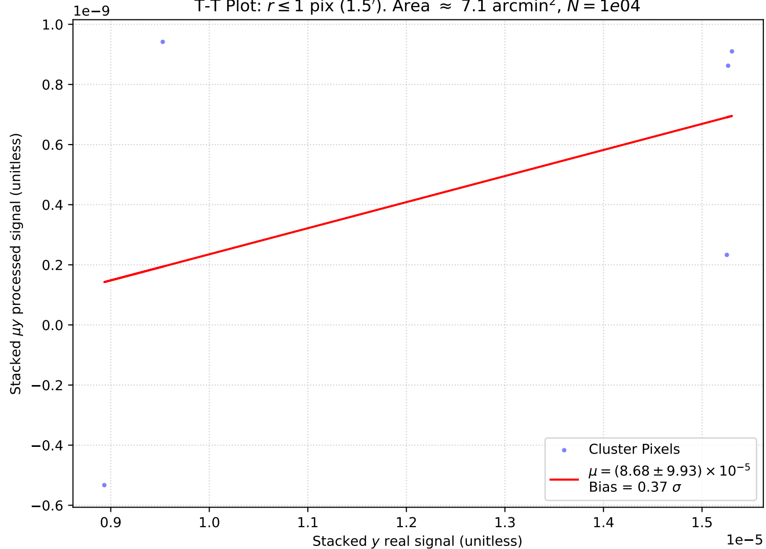
T-T Plot: r \leq 1 pix ( 1.5' ). Area \approx 7.1 arcmin 2 , N = 1e04
