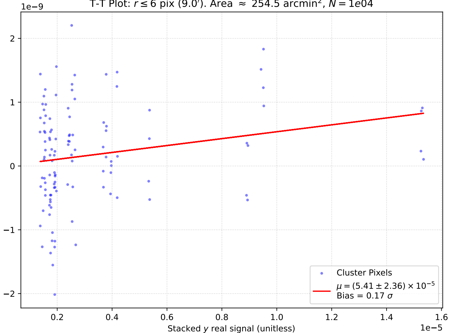
T-T Plot: r \leq 6 pix (9.0'). Area \approx 254.5 arcmin 2 , N = 1e04
