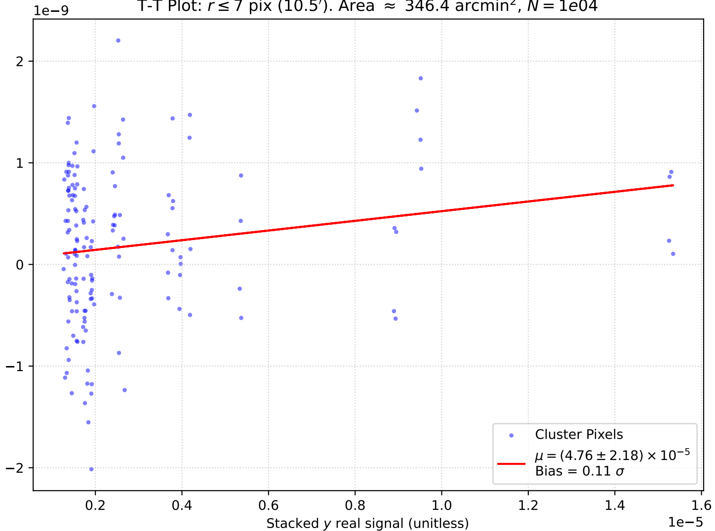
T-T Plot: r \leq 7 pix (10.5'). Area \approx 346.4 arcmin 2 , N = 1e04
