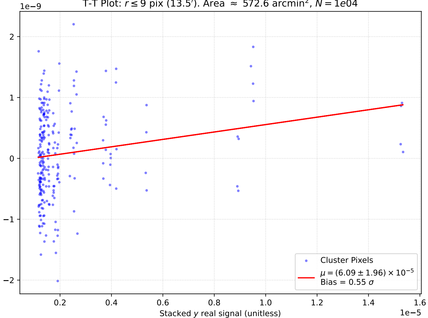
T-T Plot: r \leq 9 pix (13.5'). Area \approx 572.6 arcmin 2 , N = 1e04
