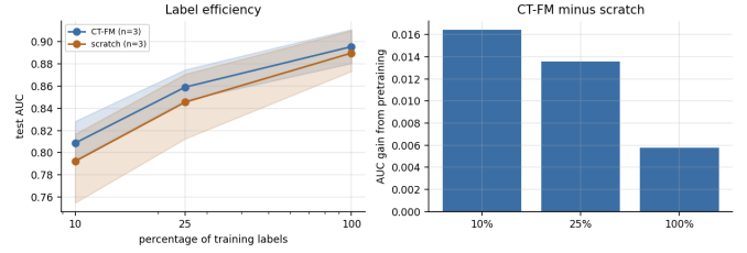
Fig. 1. Label efficiency and the mean AUC gain from pretraining. Shaded bands span the minimum and maximum over three seeds.
