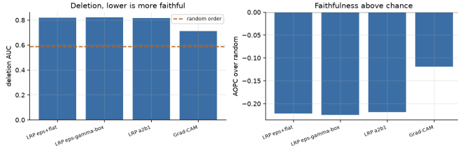
Fig. 2. Deletion AUC against the random-order baseline, and AOPC relative to random. All four attribution methods fall on the wrong side of the baseline.
