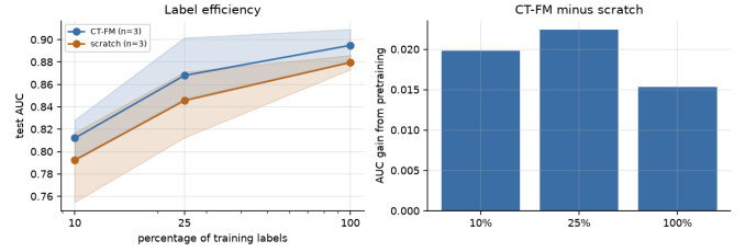
Fig. 1. Label efficiency and the AUC gain attributable to pretraining.
