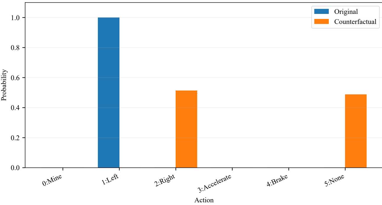
Action Probabilities Before and After
