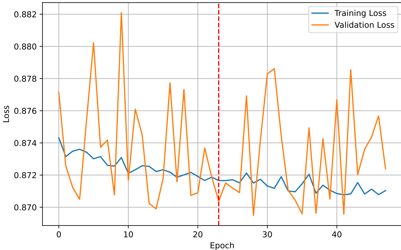
Training and Validation Loss BCE
