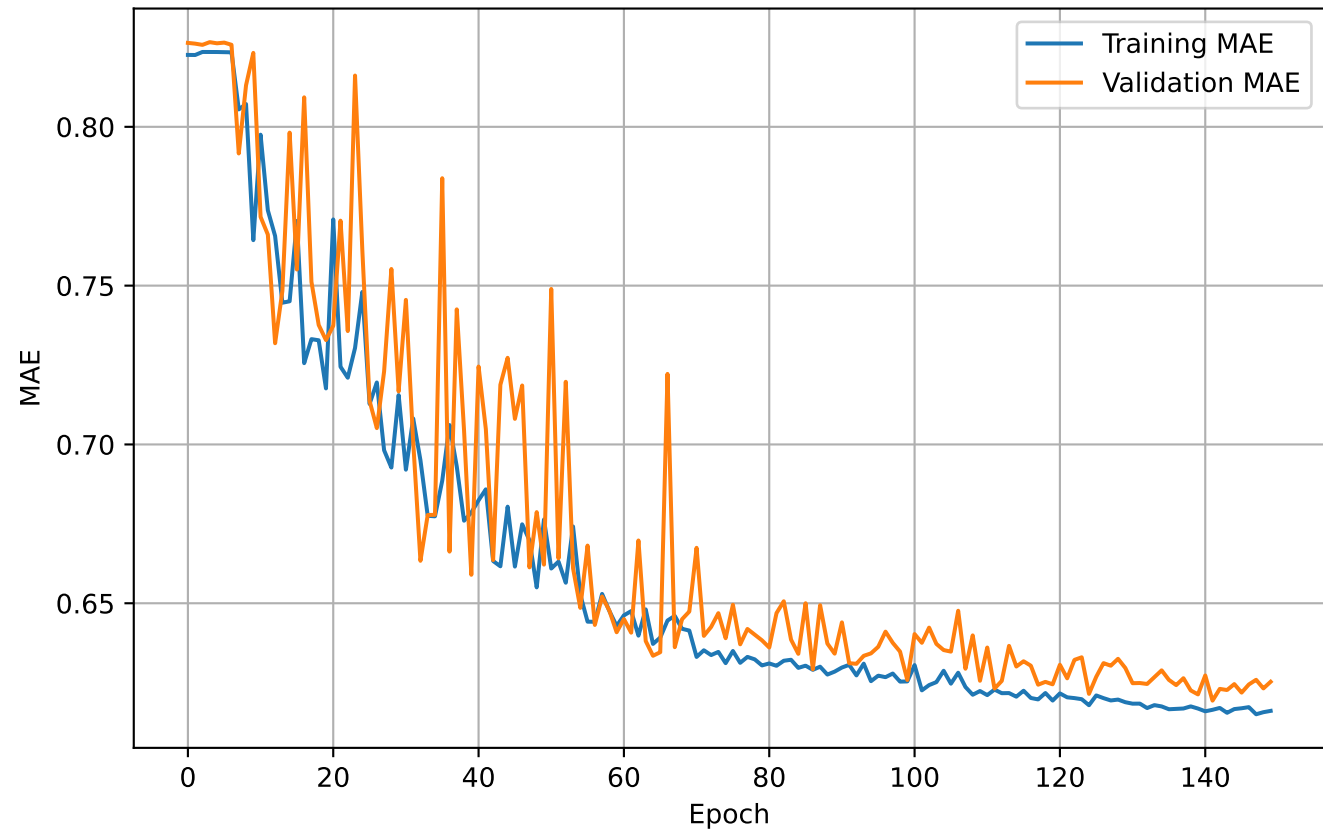
Training and Validation MAE
