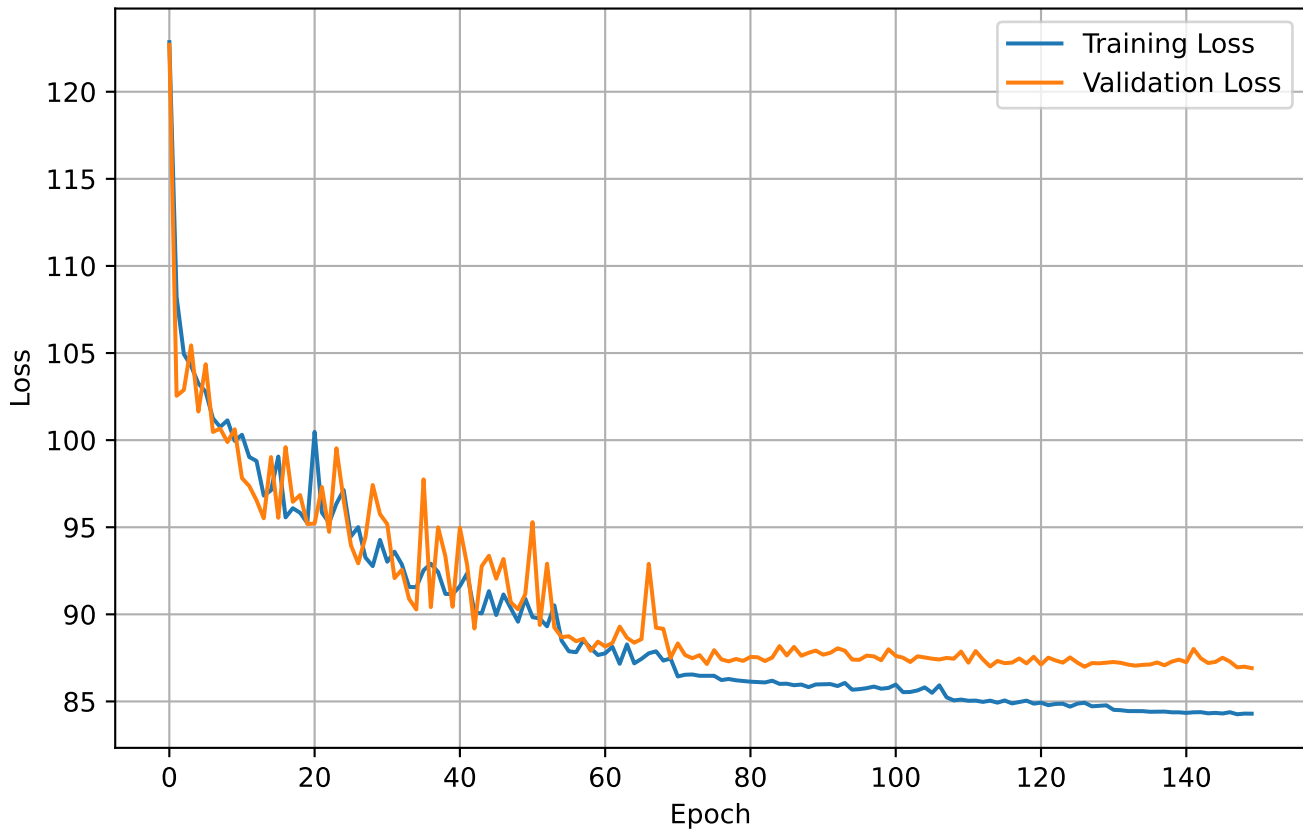
Training and Validation Loss [MAPE]
